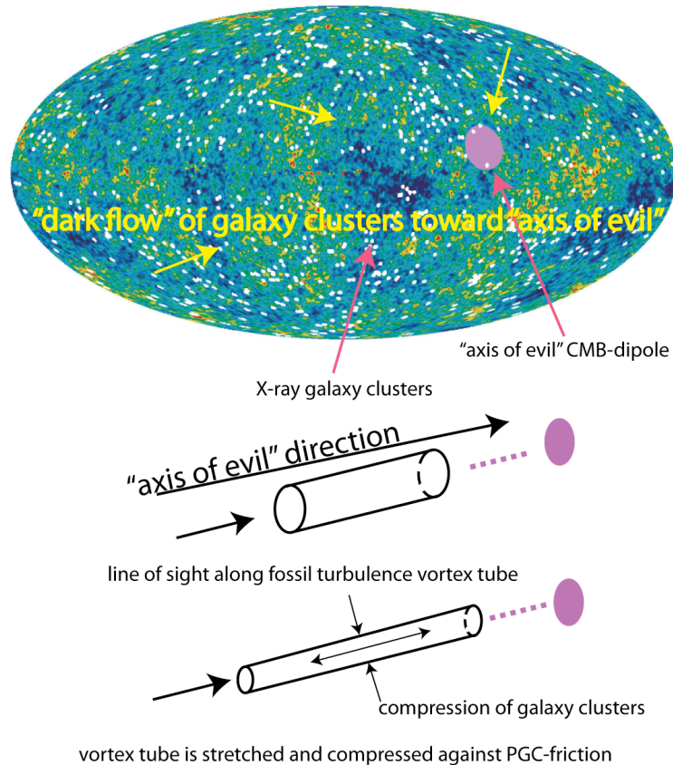
X-ray galaxy clusters moving radially toward the “axis of evil” CMB-dipole direction
